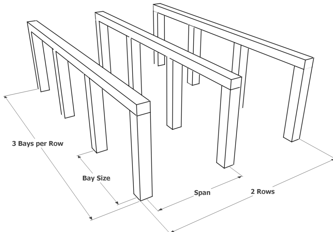
Figure 6 Bay and Span terminology
