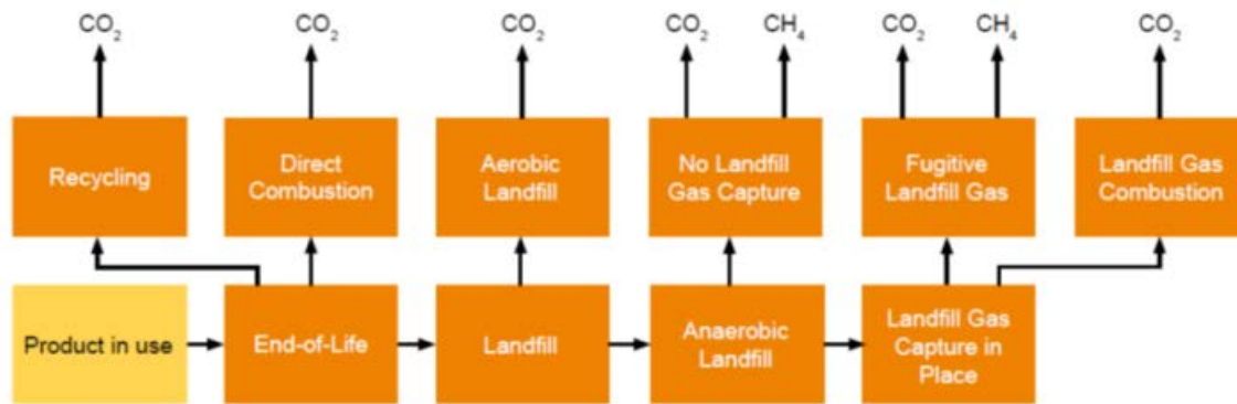
Figure 5 End-of-life model for wood products
