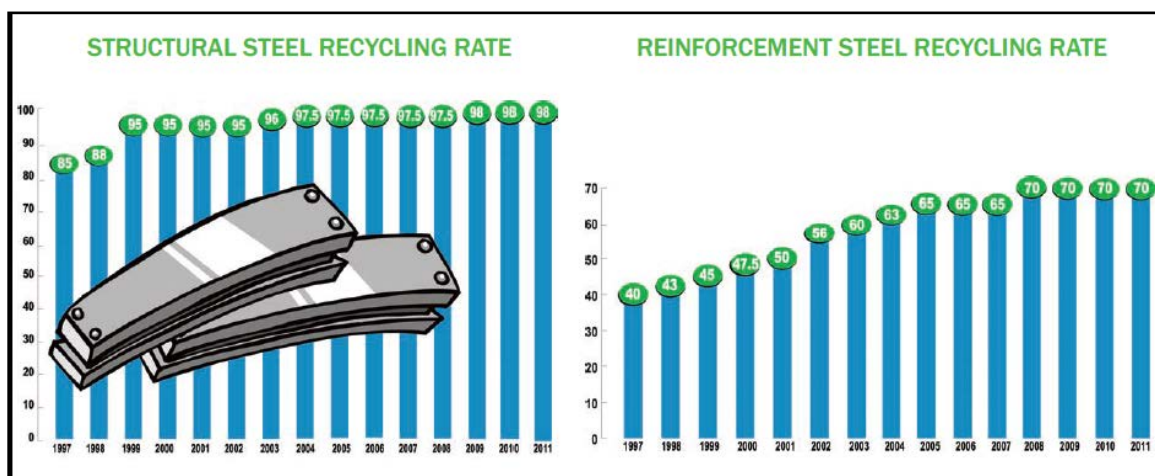
Figure 4 Recycling rates of North American steel products
